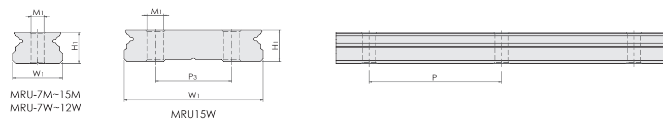
Standard MRU-M series - Tapped from bottom
