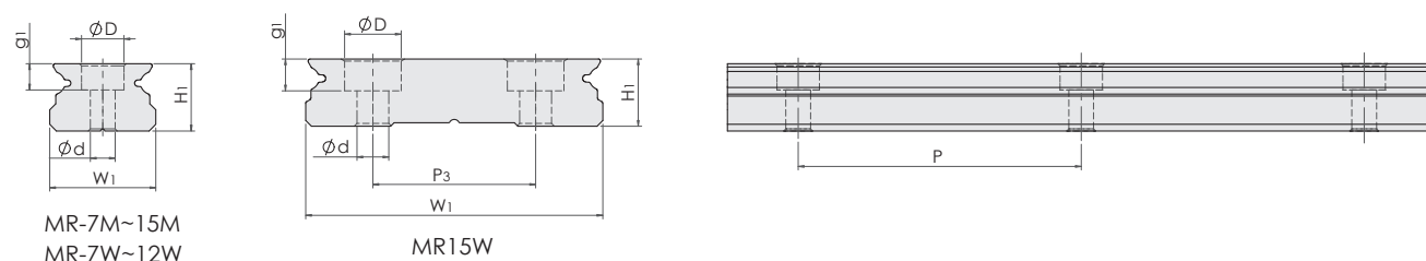
Standard MR-M series Rail
